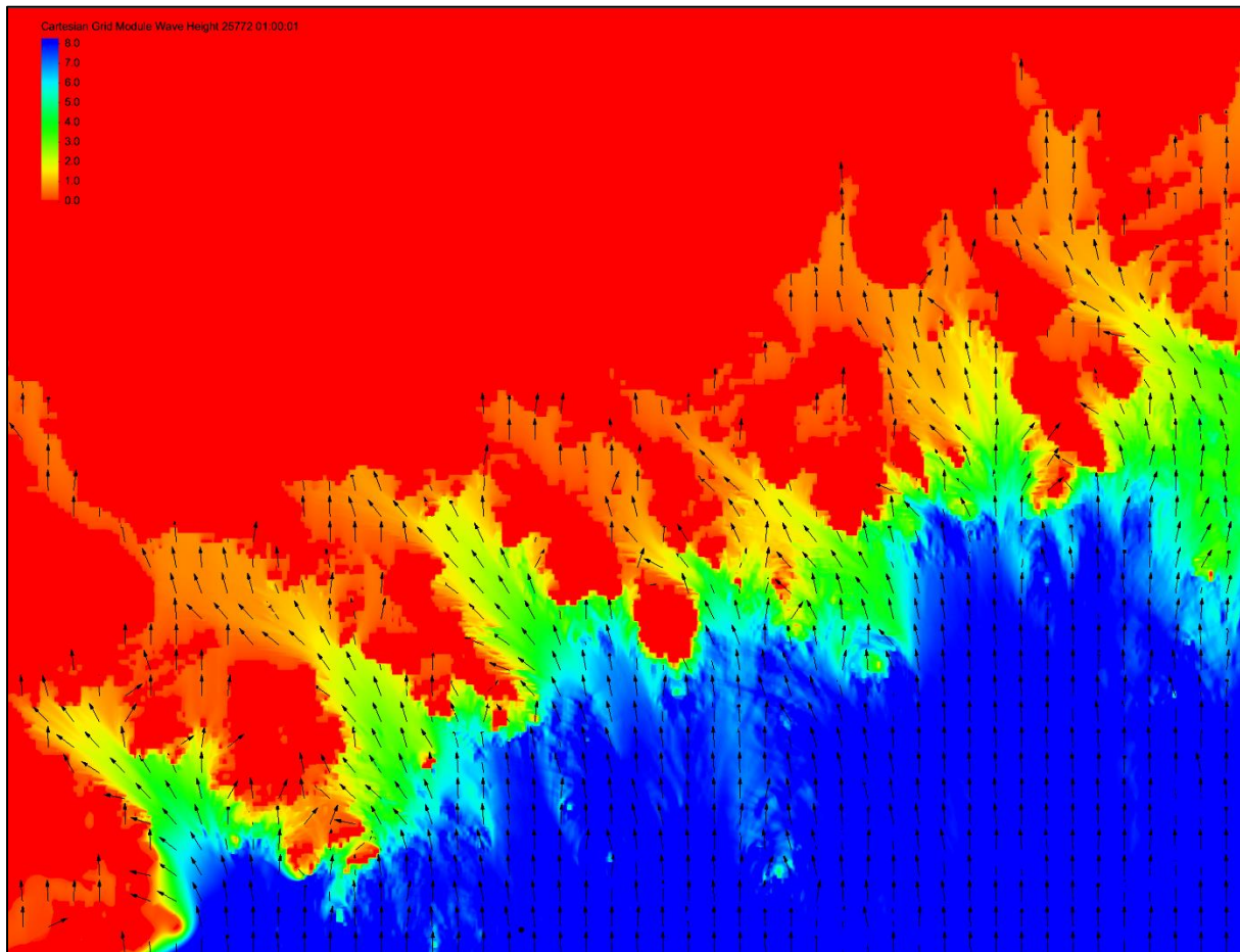
Figure 14 Wave modeling results for direction [From] 180 deg- S
