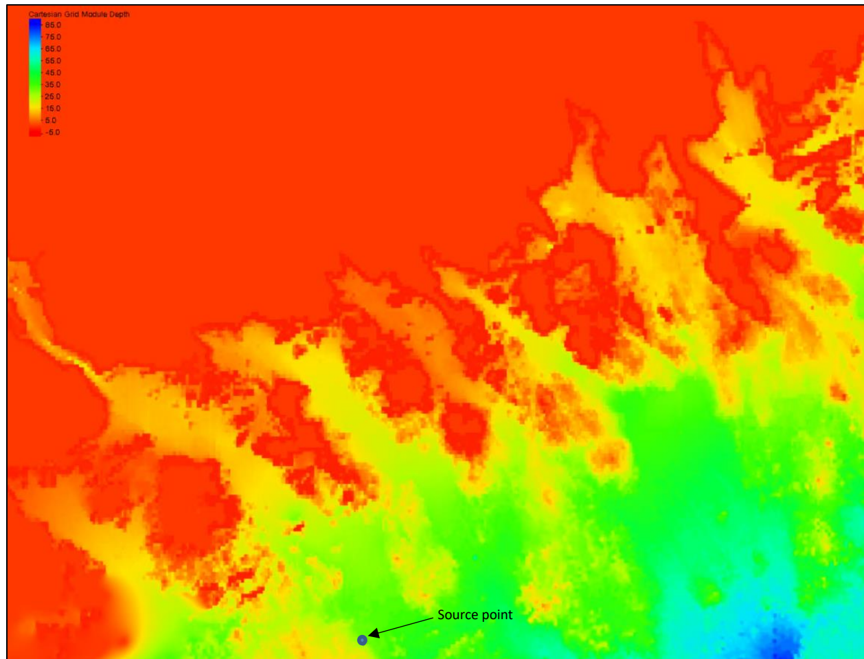
Figure 4 Bathymetry at site on STWave. Note the MSC50 HindCast model source point indicated at 44° 42.000' N, 62° 42.000' W Boundary conditions – offshore wind and wave conditions
