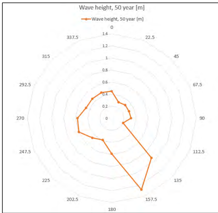
Figure 16 Maximum wave height at 50- year return period and direction [from]- Ship Harbour - Marine Finfish Lease - 0772
