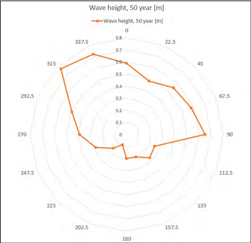
Figure 18 Maximum wave height at 50- year return period and direction [from]- Ship Harbour - Marine Finfish Lease - 0833
