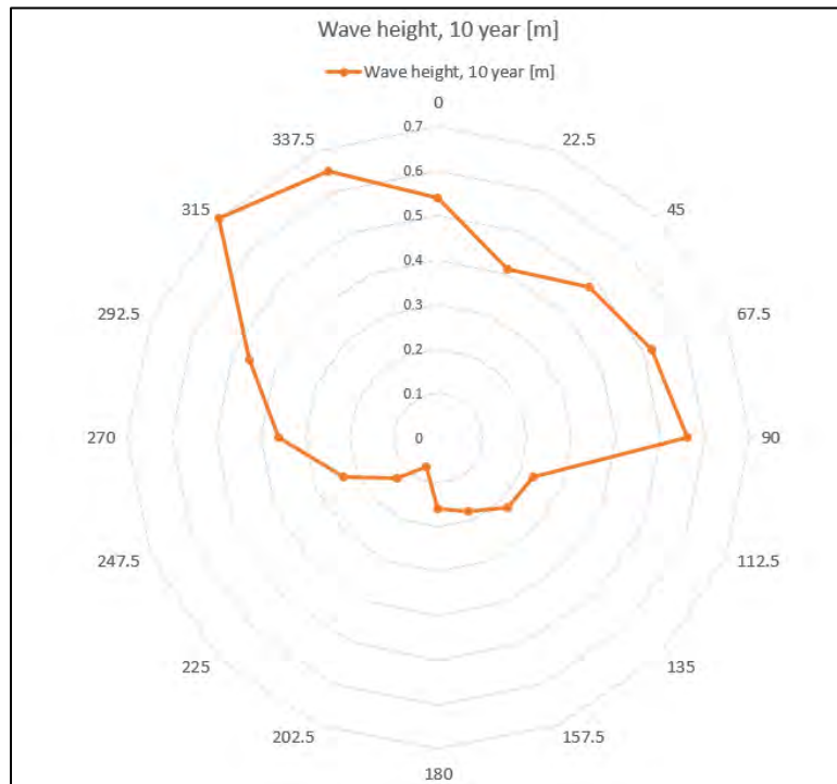
Figure 17 Maximum wave height at 10- year return period and direction [from]- Ship Harbour - Marine Finfish Lease - 0833
