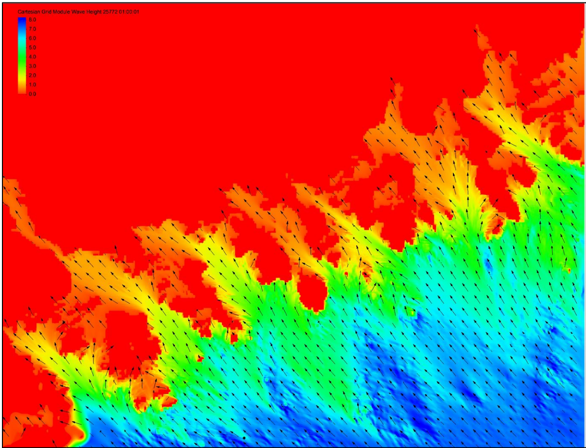
Figure 13 Wave modeling results for direction [From] 135 deg- SE
