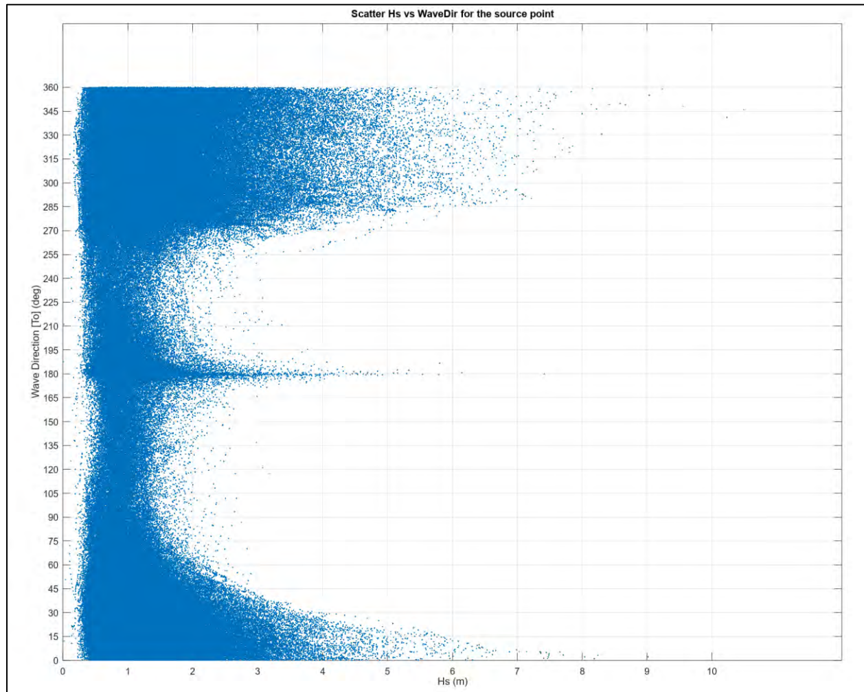
Figure 5 Wave height versus wave direction plot
