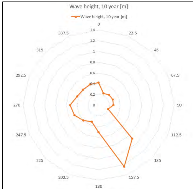
Figure 15 Maximum wave height at 10- year return period and direction [from]- Ship Harbour - Marine Finfish Lease - 0772
