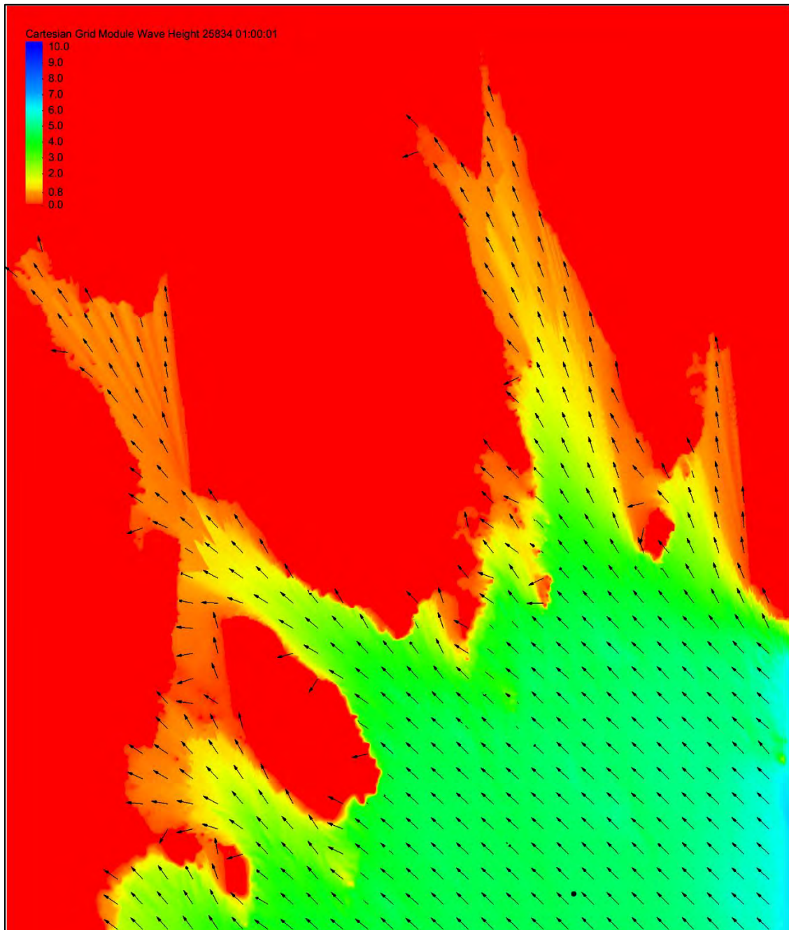
Figure 14 Wave modeling results for direction [From] 135 deg- SE
