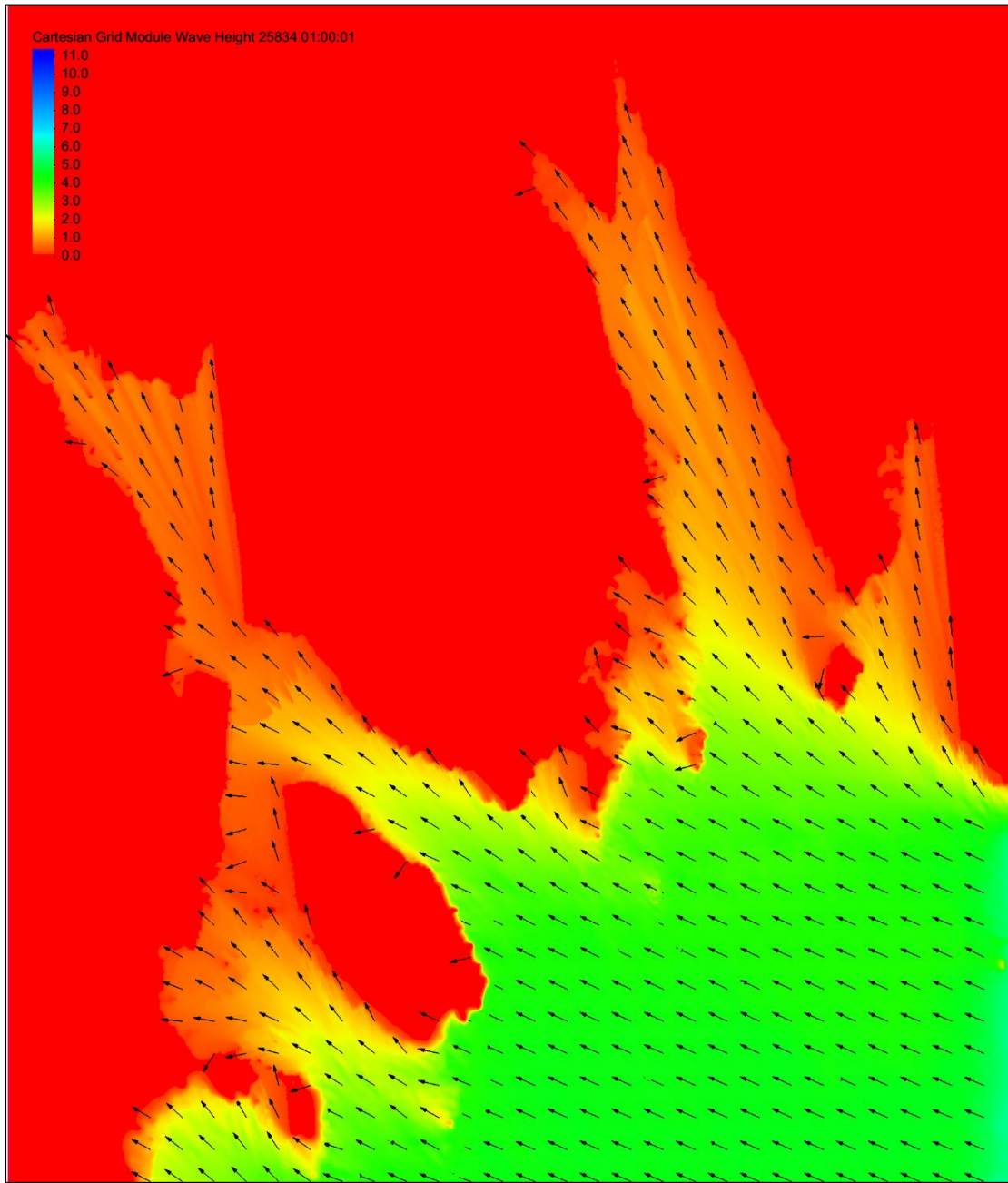
Figure 13 Wave modeling results for direction [From] 113 deg- ESE
