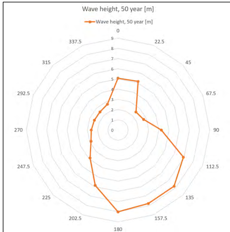
Figure 12 Maximum wave height at 50- year return period and direction [from]- for Source Point offshore location [1]
