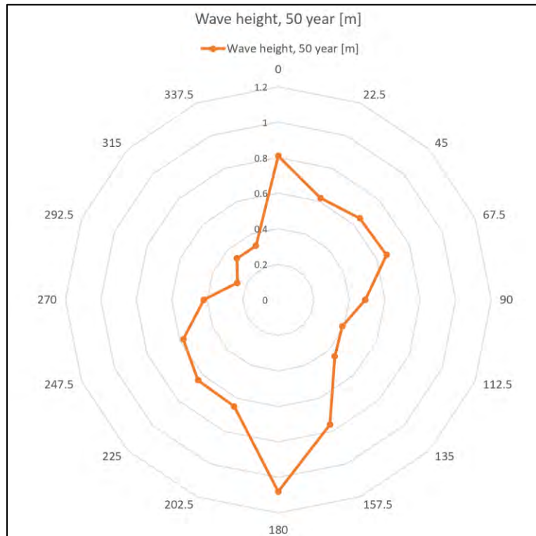
Figure 20 Maximum wave height at 50- year return period and direction [from]- Shelburne Harbour - Marine Finfish Lease - 1192
