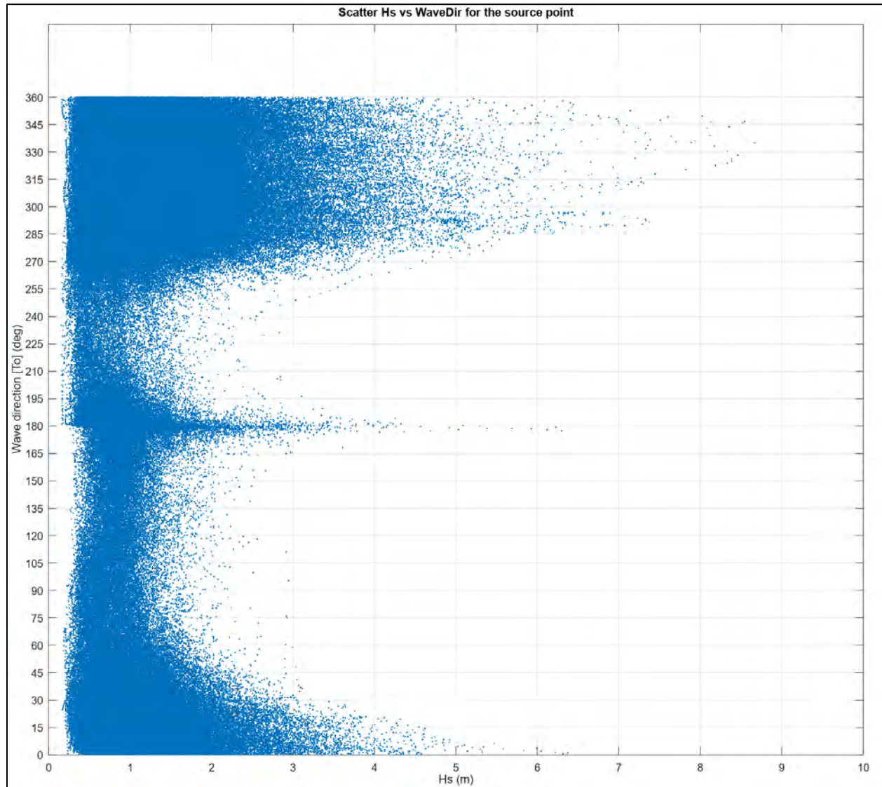
Figure 5 Wave height versus wave direction plot
