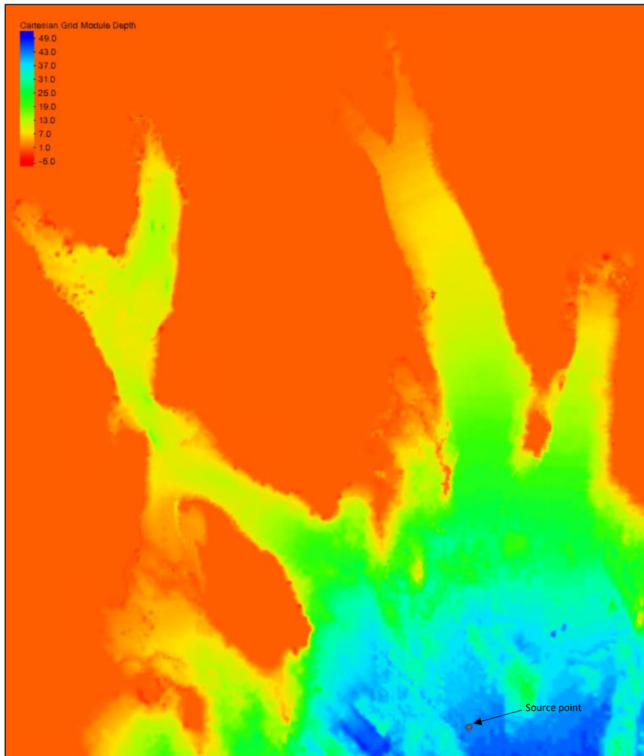
Figure 4 Bathymetry at site on STWave. Note the MSC50 HindCast model source point indicated at 43° 36.000' N, 65° 12.000' W Boundary conditions – offshore wind and wave conditions
