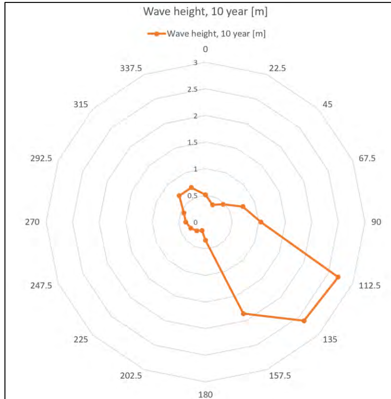
Figure 15 Maximum wave height at 10- year return period and direction [from]- Shelburne Harbour - Marine Finfish Lease - 1345
