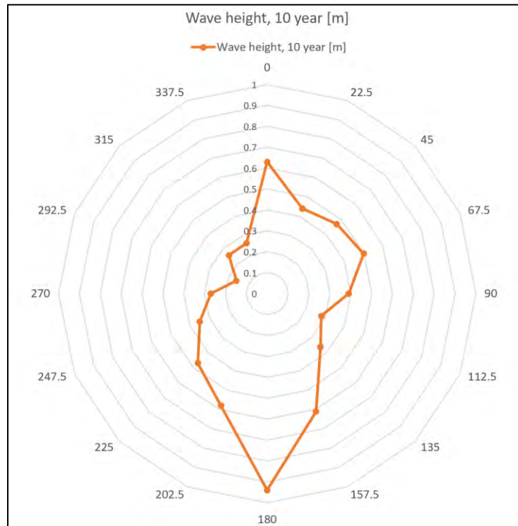
Figure 21 Maximum wave height at 10- year return period and direction [from]- Shelburne Harbour - Marine Finfish Lease – 0983
