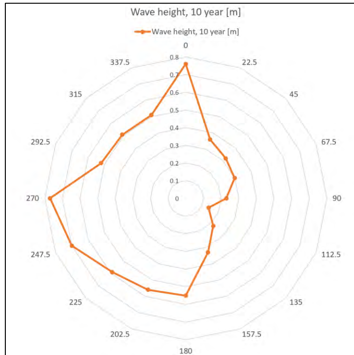
Figure 17 Maximum wave height at 10- year return period and direction [from]- Shelburne Harbour - Marine Finfish Lease – 0602
