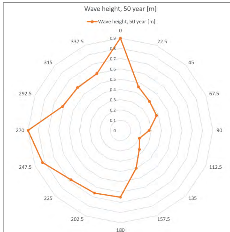
Figure 18 Maximum wave height at 50- year return period and direction [from]- Shelburne Harbour - Marine Finfish Lease – 0602
