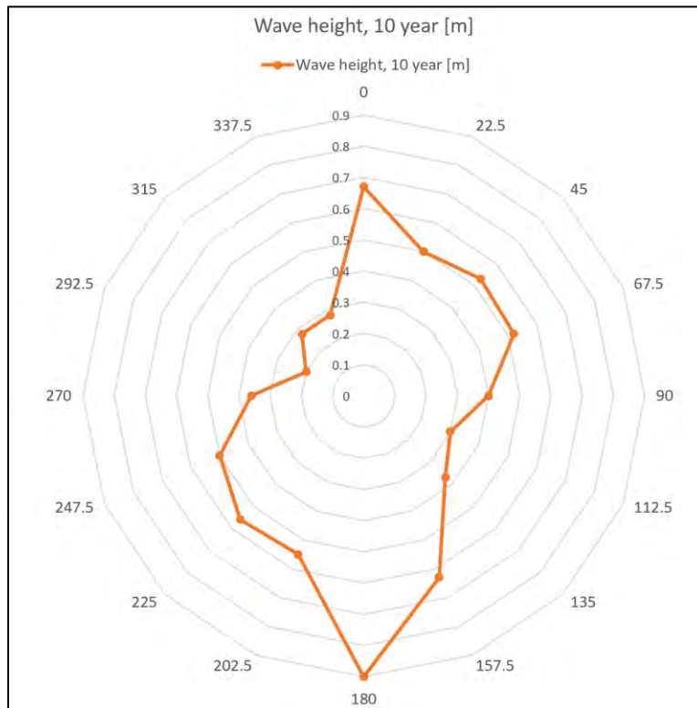
Figure 19 Maximum wave height at 10- year return period and direction [from]- Shelburne Harbour - Marine Finfish Lease – 1192
