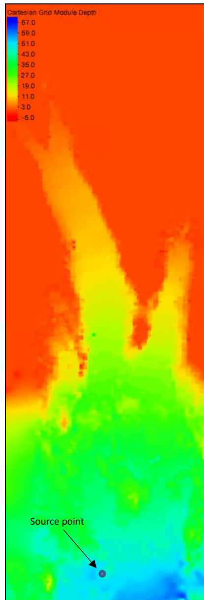
Figure 4 Bathymetry at site on STWave. Note the MSC50 HindCast model source point indicated at 43° 36.000'N, 65° 12.000'W
