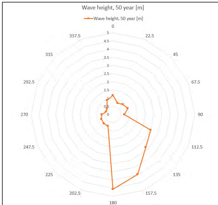
Figure 19 Maximum wave height at 50 year return period and direction [from]- Jordan Bay- Marine Finfish Lease- 1359
