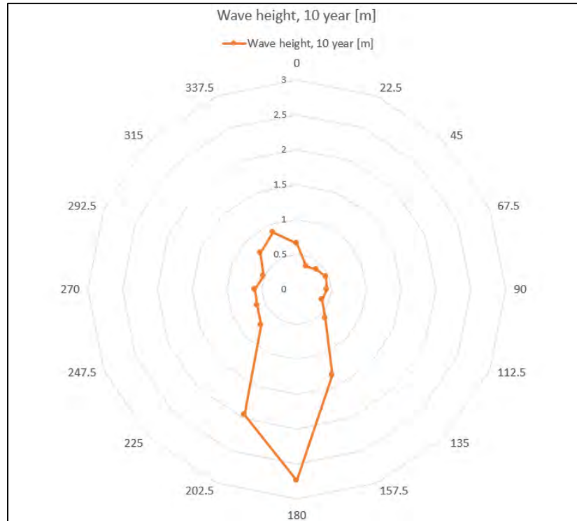
Figure 16 Maximum wave height at 10 year return period and direction [from]- Jordan Bay- Marine Finfish Lease- 1358
