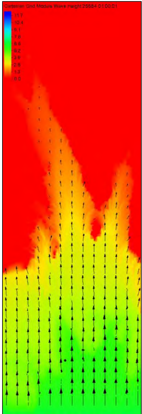
Figure 14 Wave modeling results for direction [From] 180 deg- S
