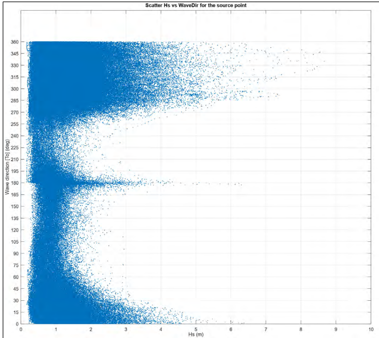
Figure 5 Wave height versus wave direction plot for the source point
