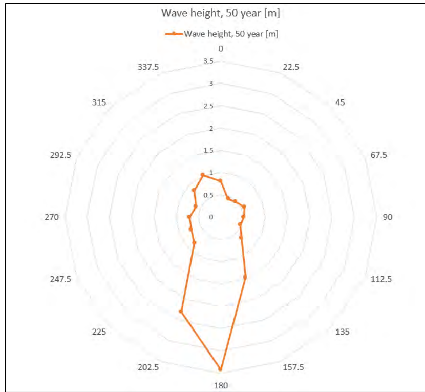
Figure 17 Maximum wave height at 50 year return period and direction [from]- Jordan Bay- Marine Finfish Lease- 1358
