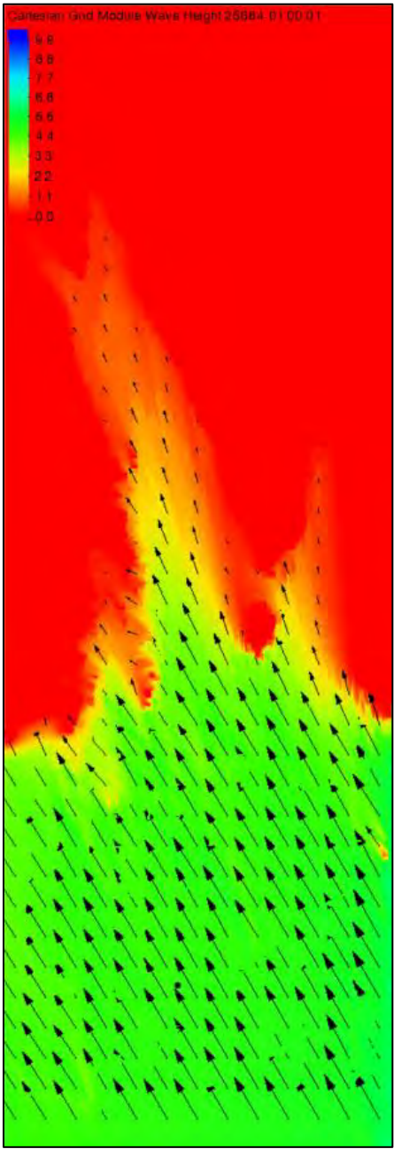
Figure 13 Wave modeling results for direction [From] 158 deg- SE
