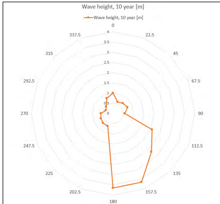
Figure 18 Maximum wave height at 10 year return period and direction [from]- Jordan Bay- Marine Finfish Lease- 1359
